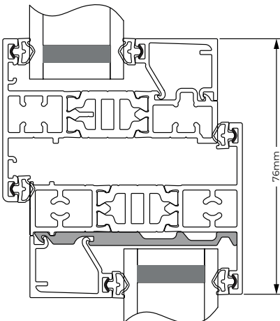
DOUBLE GLAZED BEADED CONTEMPORARY SASH NEXT TO FIXED LIGHT
