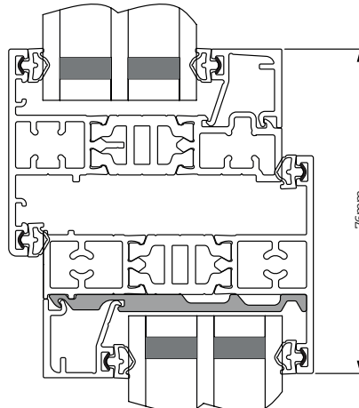
TRIPLE GLAZED BEADED CONTEMPORARY SASH NEXT TO FIXED LIGHT
