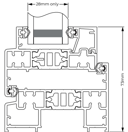
BEADED STEPPED SASH IN FLUSH INTERMEDIATE OUTER FRAME
