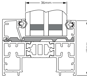
INTERMEDIATE TRIPLE GLAZED FIXED LIGHT
