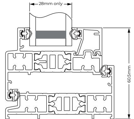
BEADED STEPPED SASH IN FLUSH SMALL OUTER FRAME
