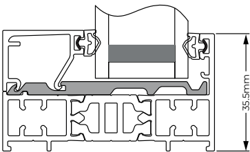
SLIM DOUBLE GLAZED FIXED LIGHT
